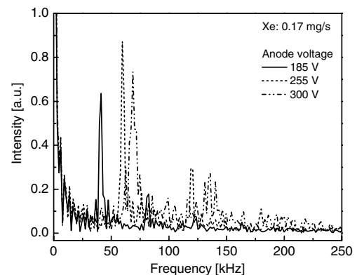
Fig. 7 Low-frequency spectral analysis of the discharge current.
