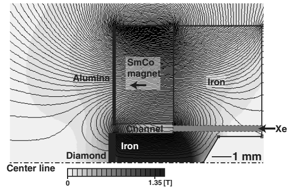
Fig. 3 Simulations of the micro-Hall thruster vacuum magnetic field.
